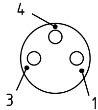
FEMALE END VIEW
