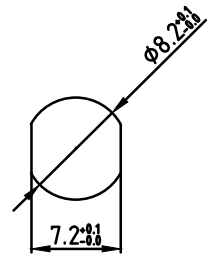
SUGGESTED PANEL CUT OUT
